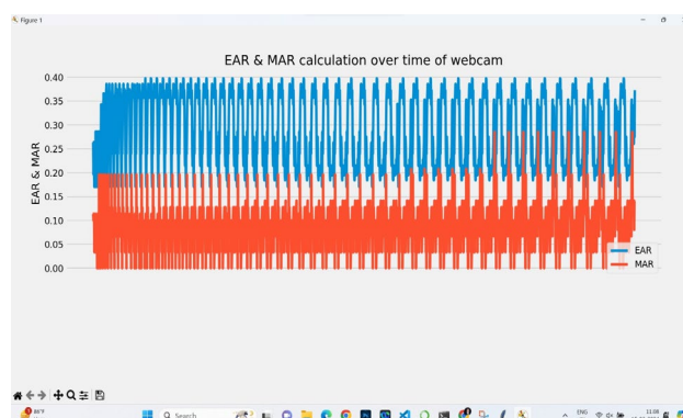
Fig. 5. EAR & MAR calculation over time of webcam
