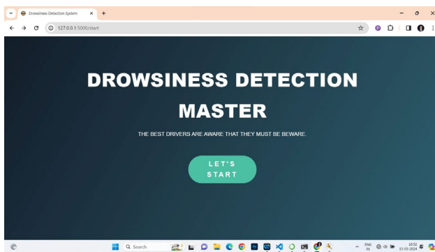
Fig. 3. Landing page
