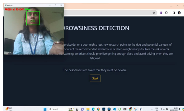
Fig. 4. Testing page
