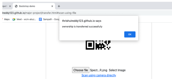
Fig. 12. Transfer ownership
