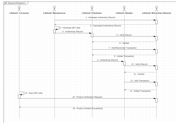
Fig. 4. Sequence diagram
