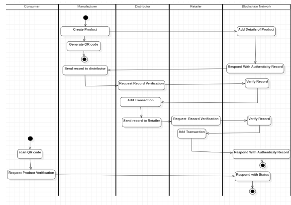
Fig. 5. Activity diagram
