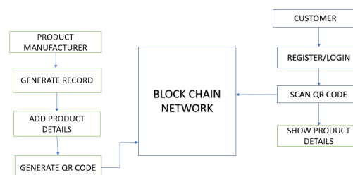
Fig. 1. System architecture
