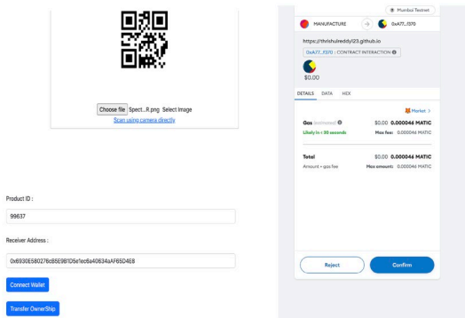
Fig. 12. Transfer ownership
