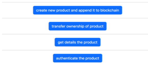
Fig. 6. Home page
