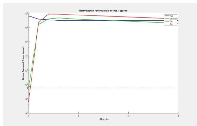
Fig. 5. Gradient descent plots
