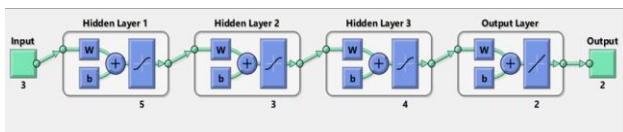
Fig. 1. Neural Network model in Matlab
